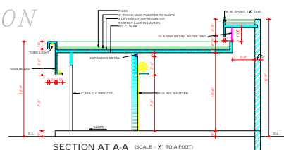
SECTION AT A-A (SCALE - X' TO A FOOT)
