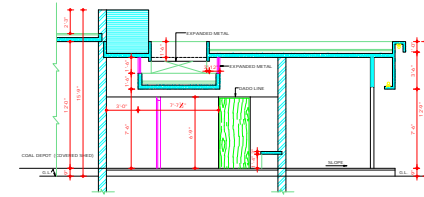
SECTION AT B-B (SCALE - X' TO A FOOT)
